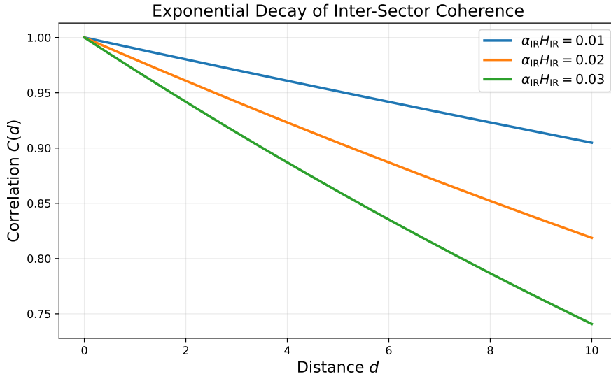
Figure 1: Exponential decay of inter-sector coherence obtained from the stationary solution of a transport–decay model. The correlation function follows C(d) \propto \exp[-d/\ell_{\text{coh}}] with \ell_{\text{coh}} = c/(\alpha_{\text{IR}} H_{\text{IR}}) . Different curves correspond to different values of the infrared decoherence rate \alpha_{\text{IR}} H_{\text{IR}} . The coherence length marks the maximal spatial range over which global quantum correlations remain dynamically relevant within a Hubble time.
